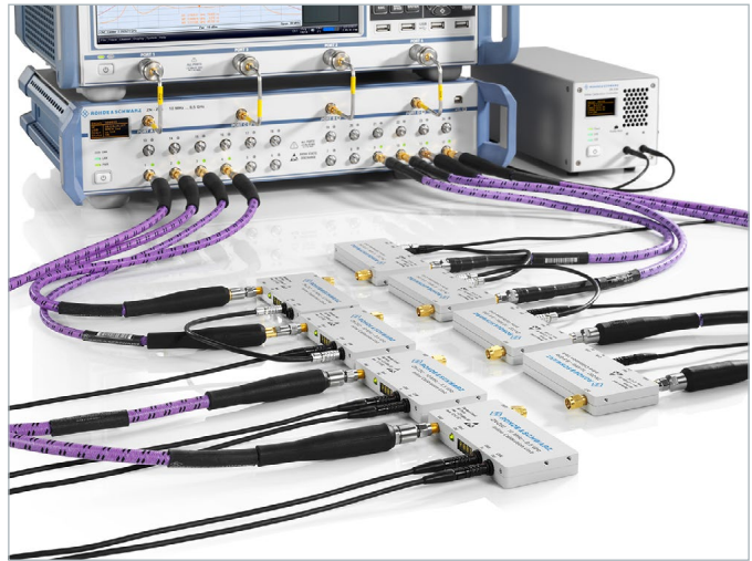
Multiport device test setup - scenario 2 (based on R&S®ZNB network analyzer, combined with a R&S®ZN-Z84 switch matrix).
